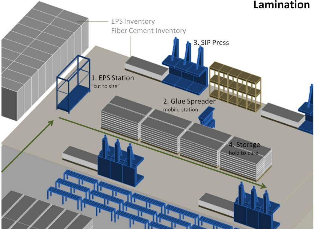
Figure 4 - Lamination
