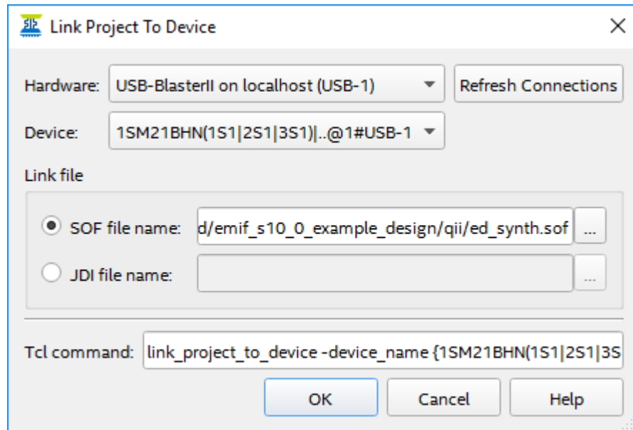
Figure 119. Link Project to Device Dialog Box
