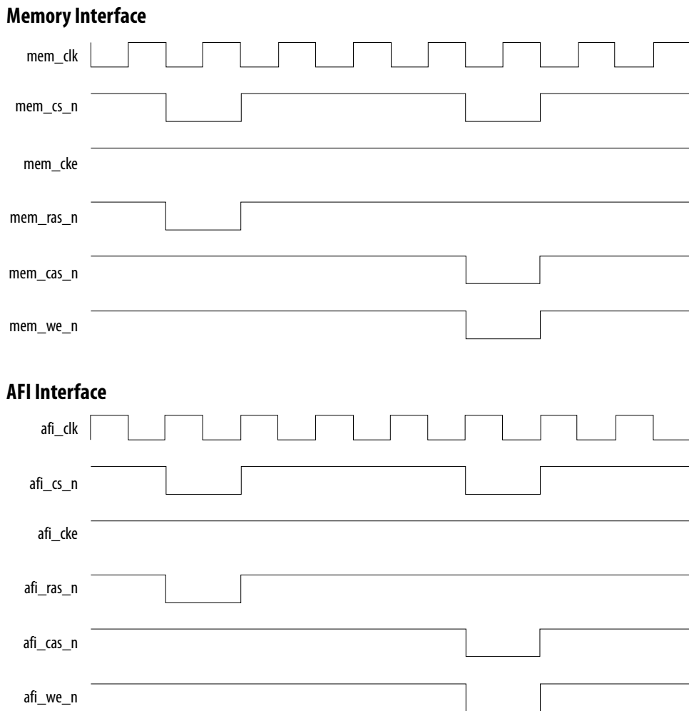
Figure 24. AFI Address and Command Full-Rate
