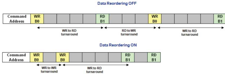
Figure 106. Data Reordering for Minimum Bus Turnaround
