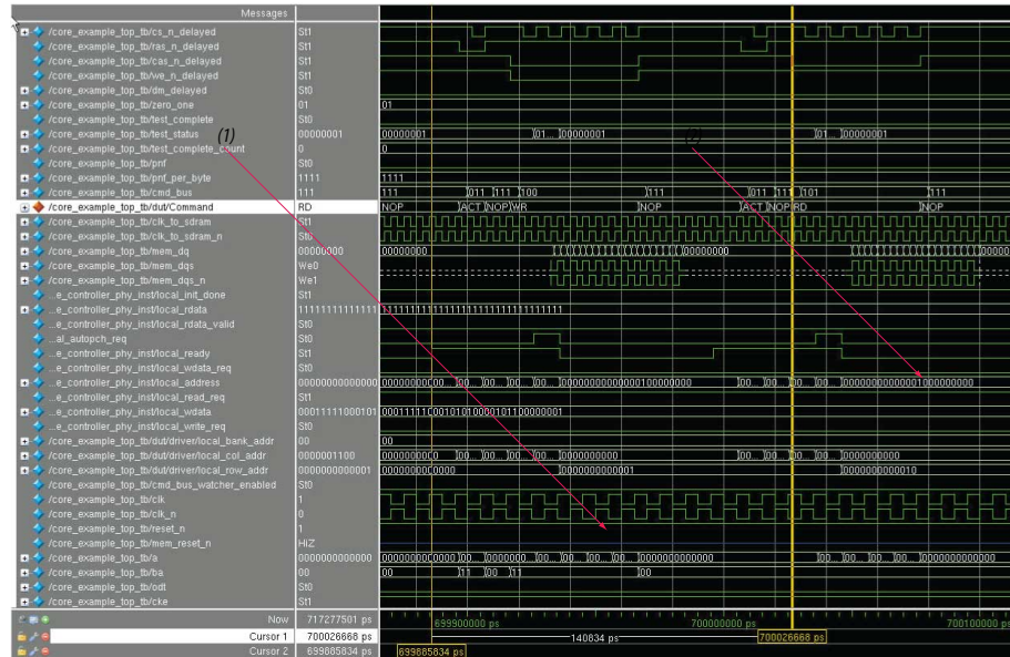
Figure 100. Improving Efficiency Using Auto-Precharge Command
