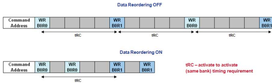
Figure 107. Data Reordering for Minimum t_{RC}
