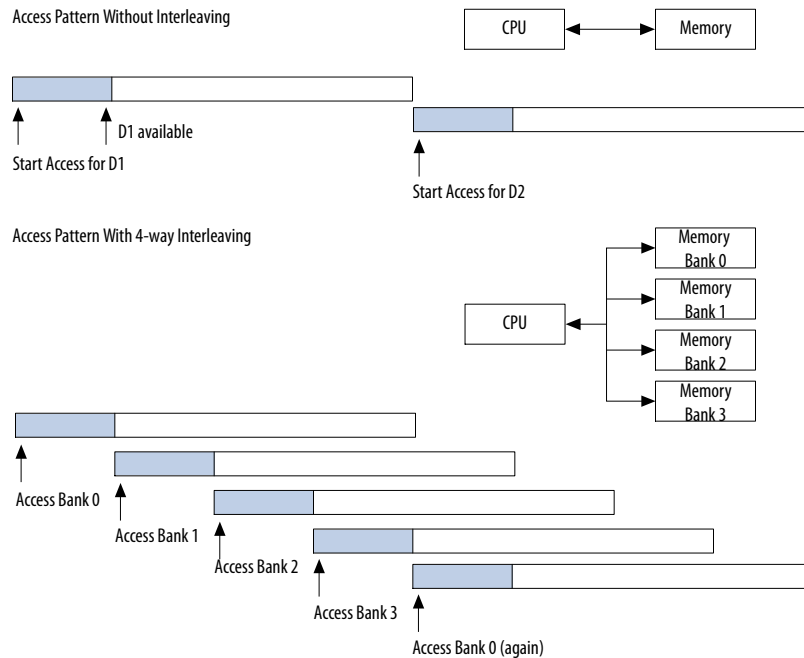
Figure 102. Using Interleaving to Increase Bandwidth
