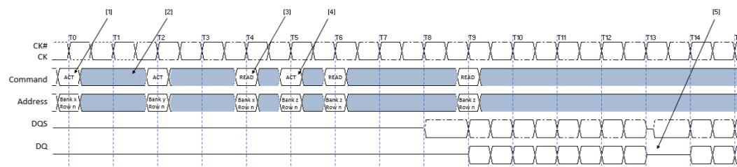
Figure 103. Bank Interleaving—Without Additive Latency
