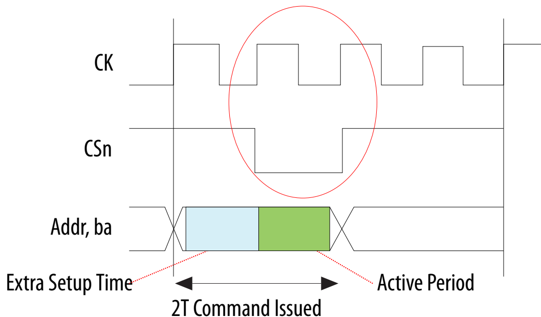
Figure 18. 2T Command Timing
