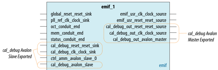
Figure 116. EMIF With Both cal_debug Master and Slave Exported
