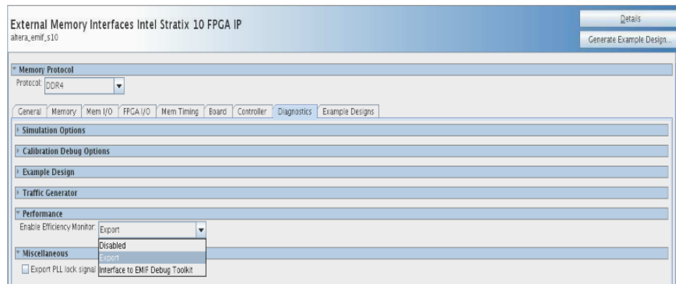
Figure 123. Enabling the Efficiency Monitor and Protocol Checker
