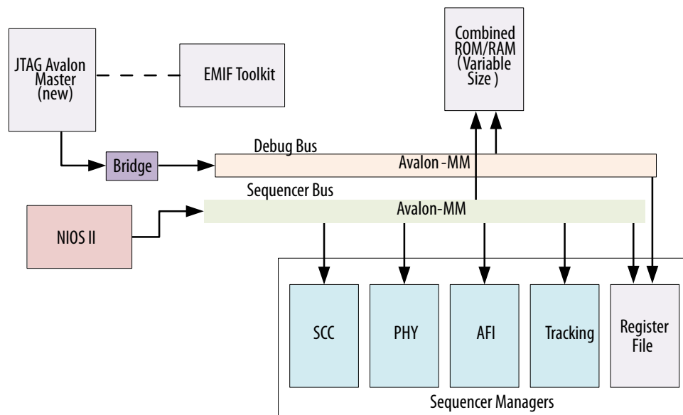
Figure 118. EMIF IP with JTAG Avalon-MM Master
