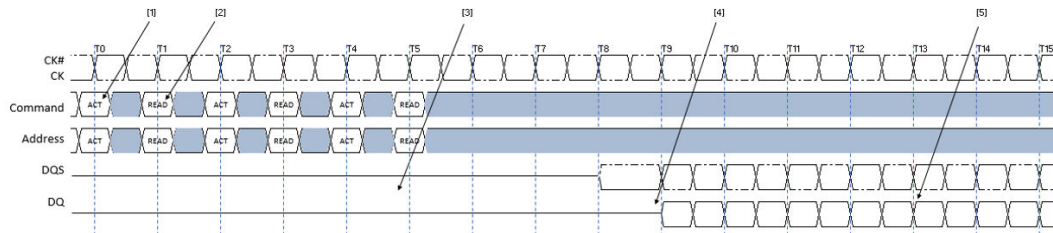
Figure 104. Bank Interleaving—With Additive Latency
