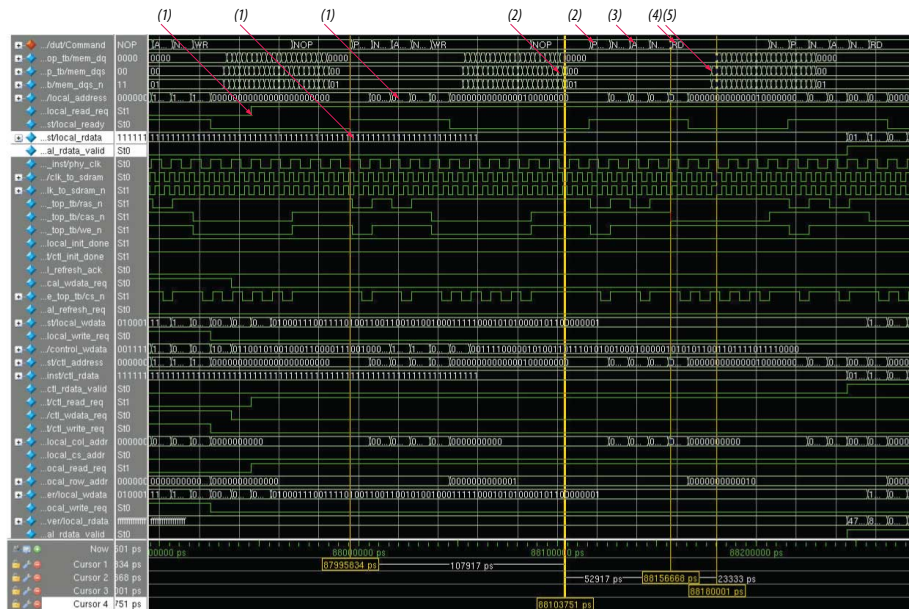
Figure 96. Read Operation—Changing A Row in A Bank
