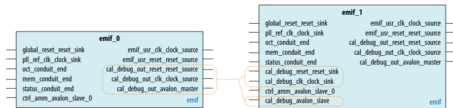
Figure 117. EMIF Components Connected
