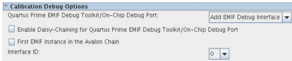
Figure 112. UDIMM DDR4 IP - Calibration Debug Options
