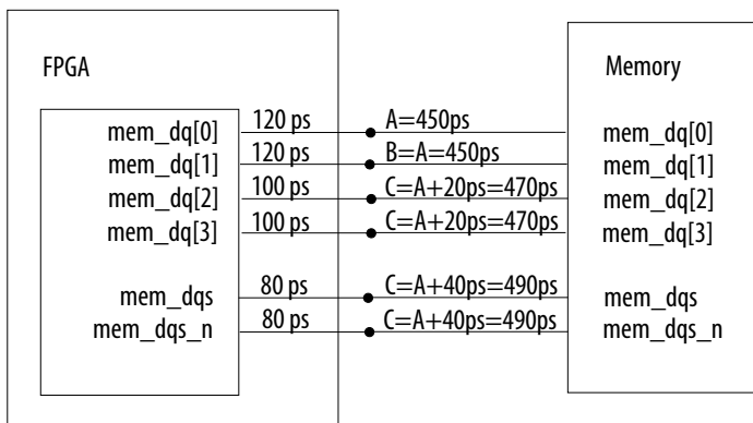
Figure 57. Deskew Example with Trace Delay Calculations
