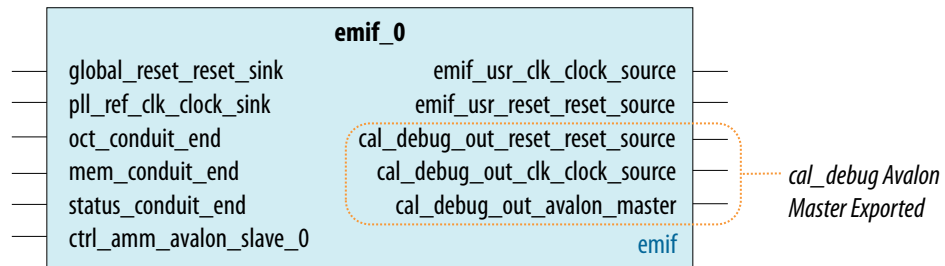
Figure 114. EMIF With cal_debug Avalon Master Exported
