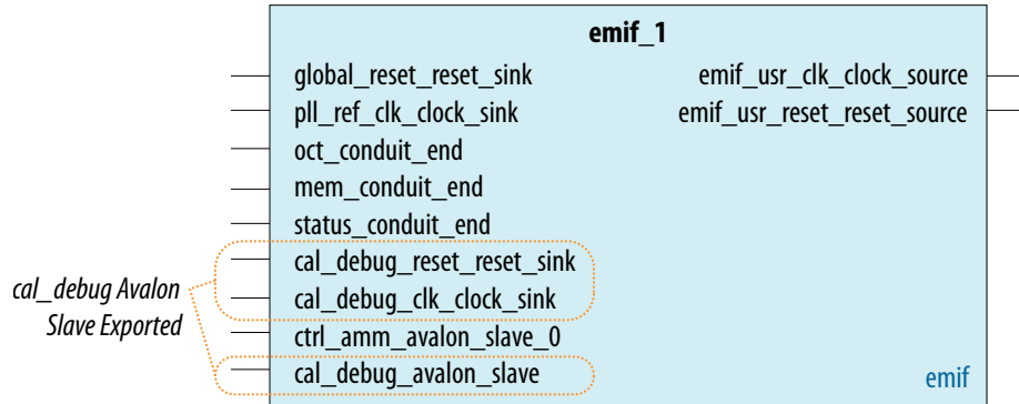
Figure 115. EMIF With cal_debug Avalon Slave Exported
