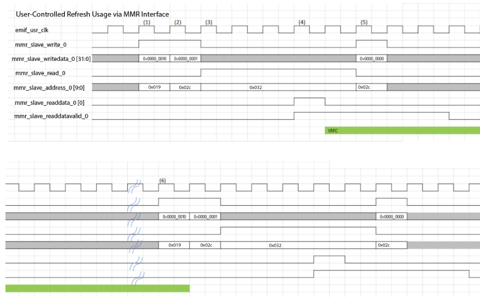
Figure 105. User-Controlled Refresh via MMR Interface
