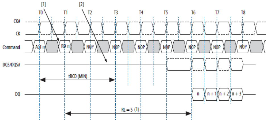
Figure 101. Additive Latency—Read
