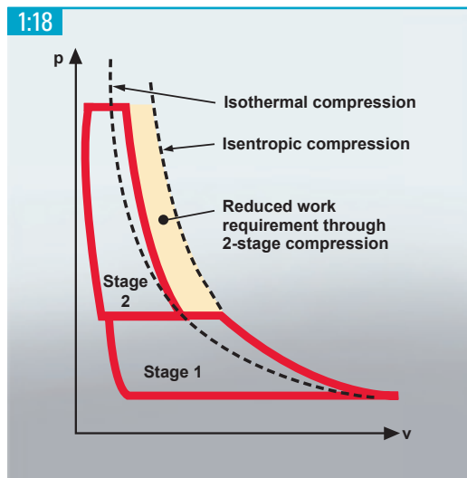
The colored area represents the work saved by dividing compression into two stages.
