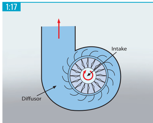
Radial turbocompressor.
