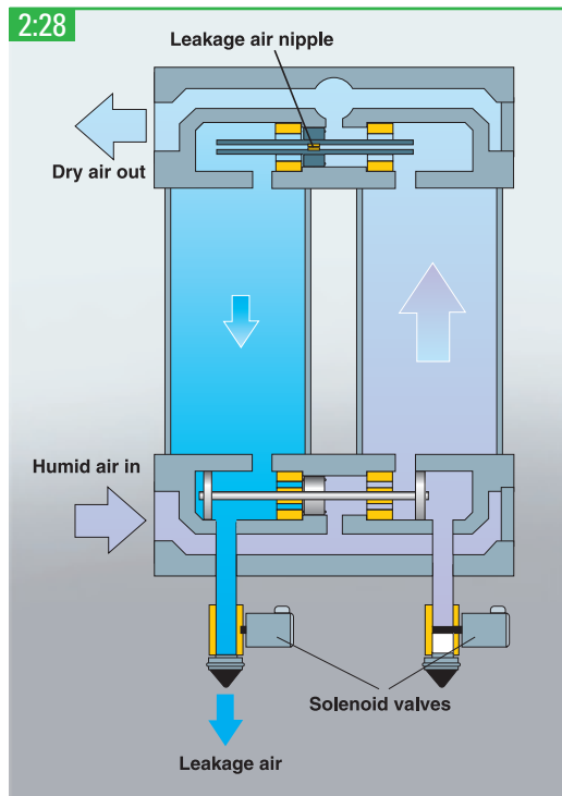
2:28 Purge regenerated adsorption dryer (also called “heatless type dryer”).
