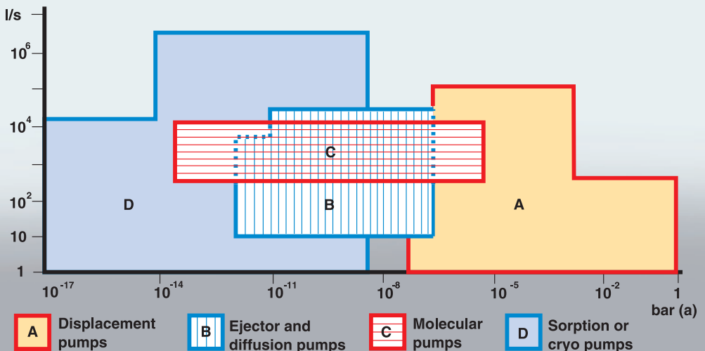
Working range for some types of vacuum pumps.
