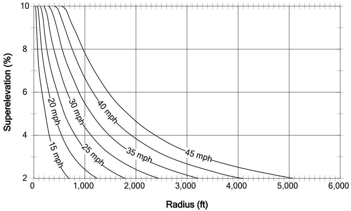
Exhibit 1250-4 Superelevation Rates (10% Max)
