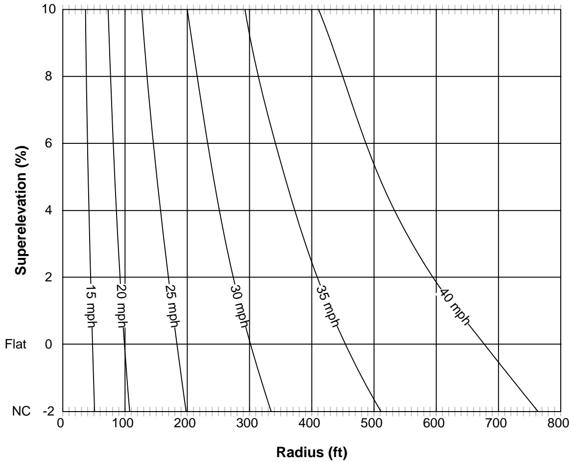
Exhibit 1250-7 Superelevation Rates for Intersections and Urban Roadways 40 mph and slower
