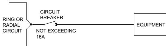
(B) CIRCUIT BREAKER PROTECTION
