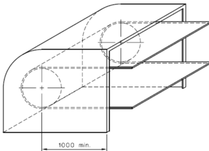
(b) Tail pulley
