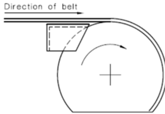
(d) Nip guard constructed from sheet metal
