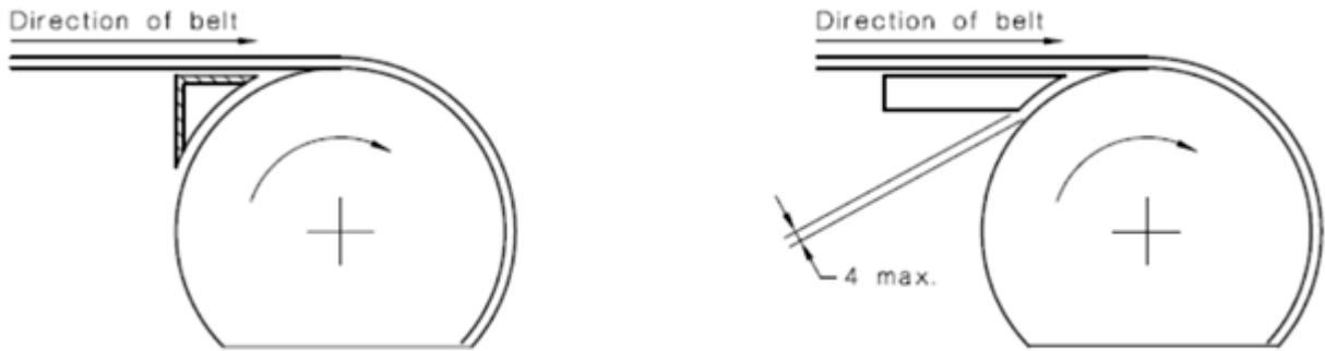
(c) Nip guard construction from rolled steel sections
