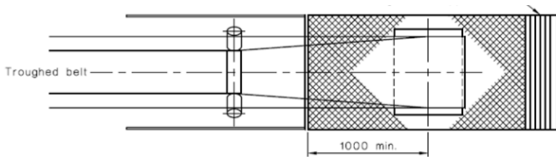
(a) Head pulley
