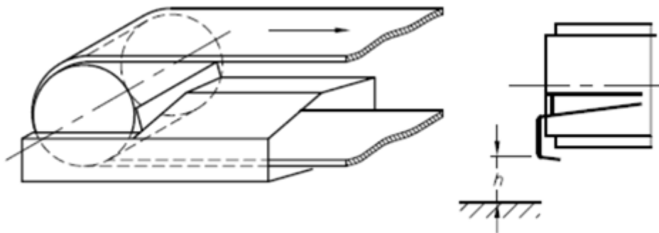
(e) Tail pulley nip guard
