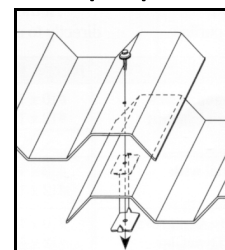
Fastening at valley w/ “No-Drip” Spacer
