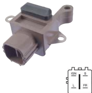
35-82088 Regulator Square, 4-Pins 150 Amp, IG-S-L-M (FR)
