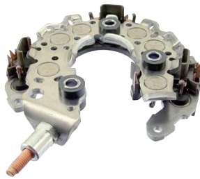
31-82052 Rectifier 117mm OD, 6mm Side Post 120-150 Amp, 12 Diodes
