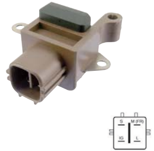
35-82089 Regulator Square, 4-Pins Amp, S-IG-L-M (FR)
