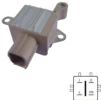
35-82086 Regulator Square, 4-Pins IG-C-L-FR
