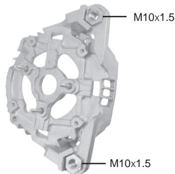
22-82102 SRE Housing 180-220 Amp, 138.5mm Stator OD
