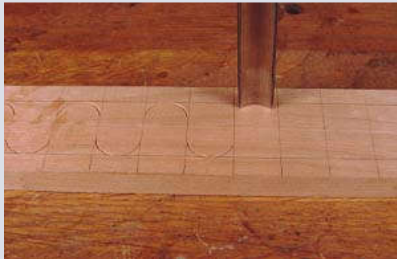
Photo 8- Using a carving gouge to establish the half circles in the carving design.
