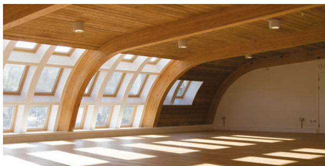
Figure 5 Horizontally laminated, curved glulam
