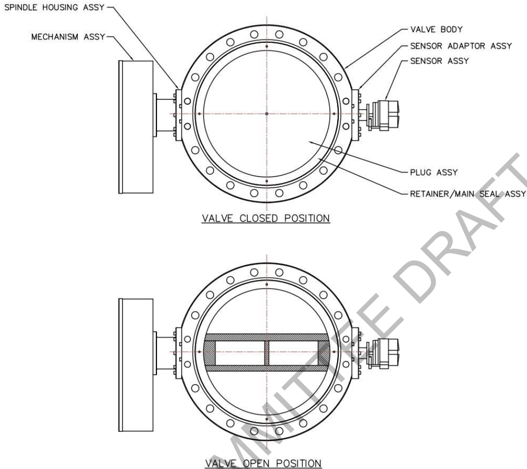
Figure 20 - Butterfly Type Pin Actuated Device
