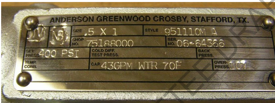
Figure 40 - Identification Tag for Pressure Relieving Device
