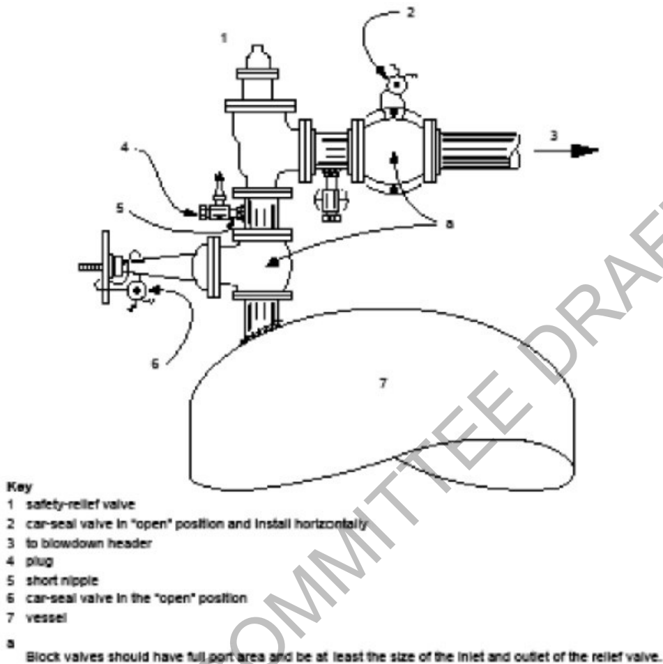
Figure 41 - Block Valves on Pressure-relief valve Inlet and Outlet Sealed Open
