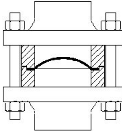
Figure 18 - Conventional Domed Rupture Disk
