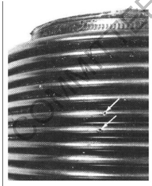
Figure 25 - Pit-type Corrosion on 18Cr-8Ni Steel Bellows
