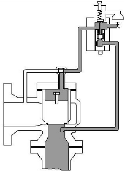
Figure 7 - Unbalanced piston main valve, Pilot-Operated Pressure-relief valve
