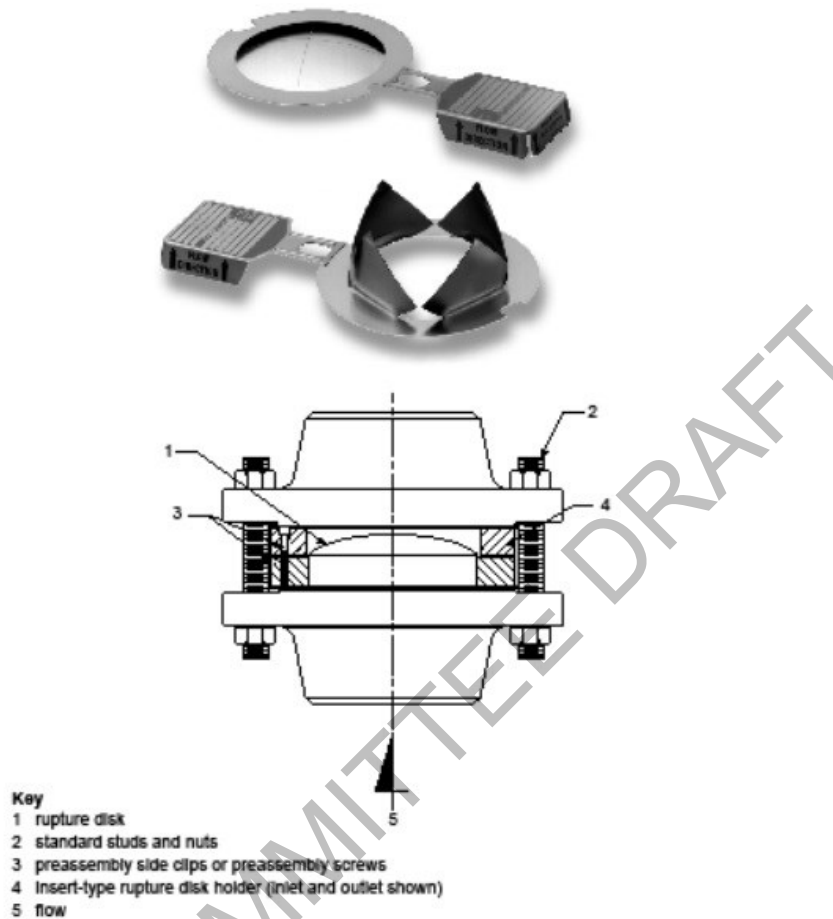
Figure 10 - Forward Acting Scored Rupture Disk
