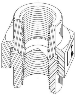
Figure 14 - Rupture Disk in union holder
