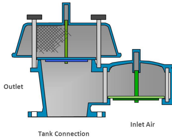
Figure 1 - Pressure/Vacuum Relief Valve
