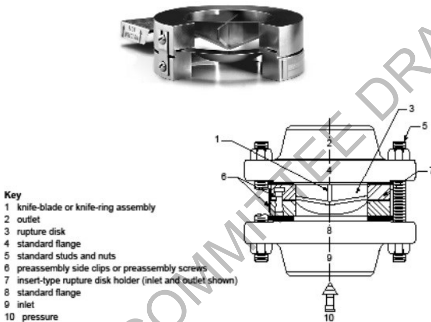
Figure 11 - Reverse Acting Knife Blade Rupture Disk
