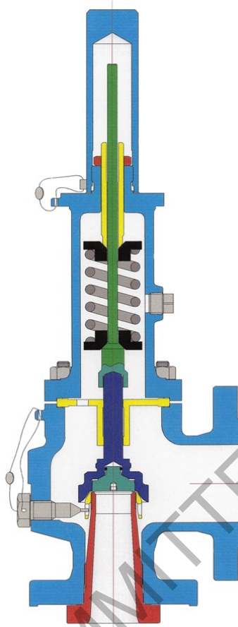
Figure 4 - Closed Bonnet, Direct Acting Spring Loaded Relief Valve
