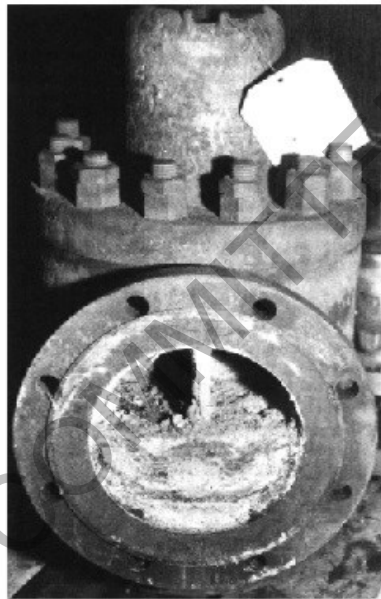
Figure 42 - Sulfur Deposits in Body of Valve
