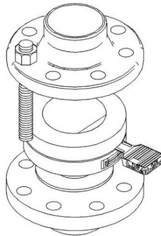
Figure 17 - Insert Type Holder Installation
