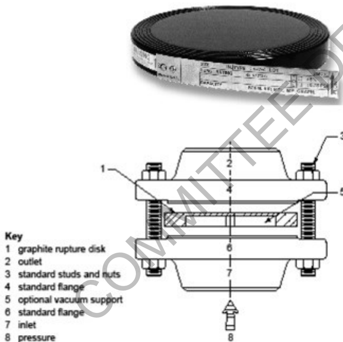
Figure 13 - Graphite Rupture Disk
