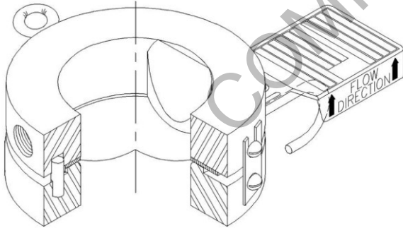
Figure 16 - Rupture Disk with Insert Type Holder
