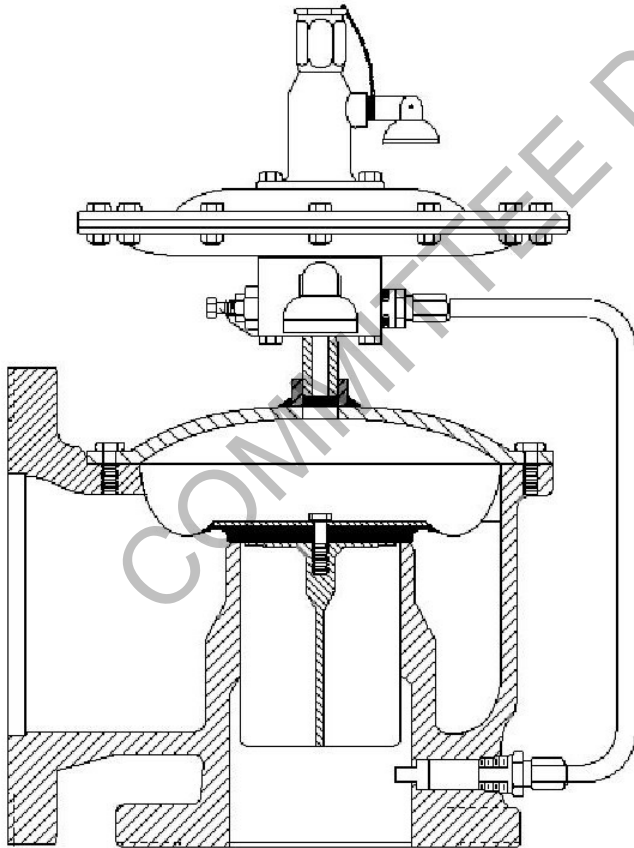
Figure 6 - Diaphragm main valve, Pilot-Operated Pressure-relief valve
