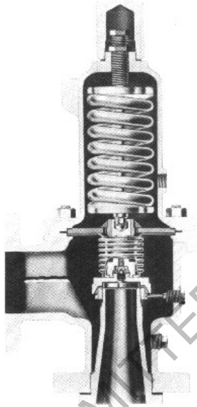
Figure 5 - Balanced Bellows Direct Acting Spring Loaded Pressure-relief valve
