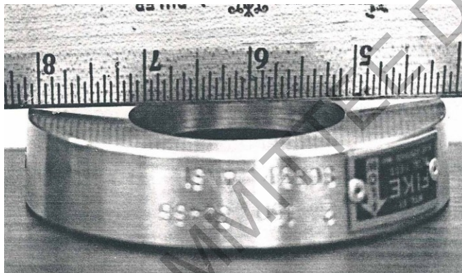
Figure 51 - Rupture Disk Holder Subjected to Over-torque
