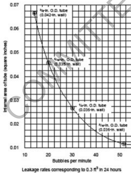
Figure 43 - Safety Valve and Relief Valve Leak Detector
