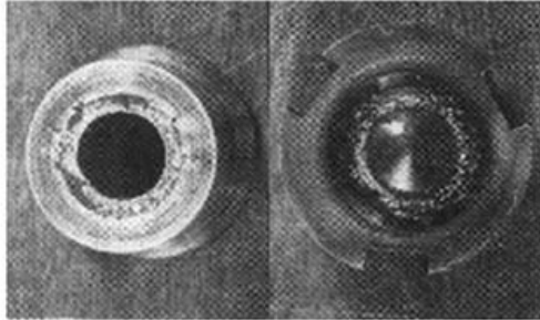
Figure 29 - Seating Surface of Disc Damaged by Frequent Operation of Valve Too Close to Operating Pressure
