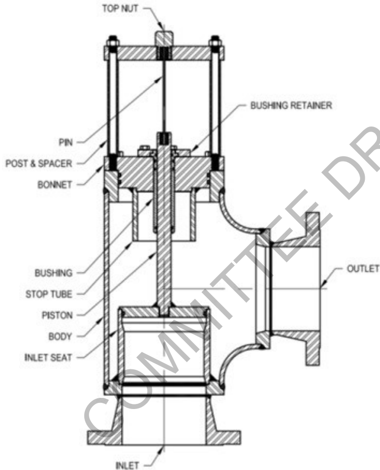
Figure 19 - Piston Type Pin Actuated Device
