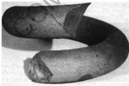
Figure 31 - Spring Failure Due to Stress Corrosion
