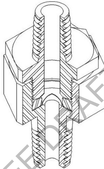
Figure 15 - Rupture Disk in Screw Type Holder
