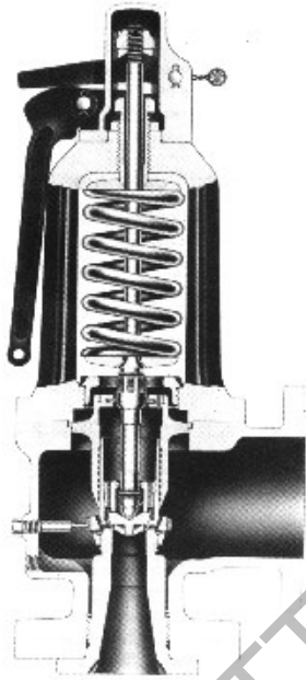
Figure 3 - Open Bonnet, Direct Acting Spring Loaded Pressure-relief valve
