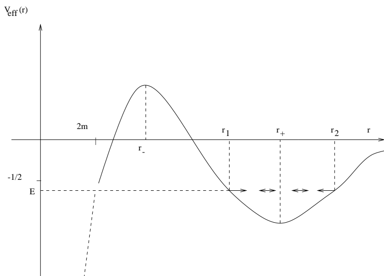
Figure 13: Effective potential for a massive particle with L/m > \sqrt{12} . Shown are the maximum of the potential at r_- (an unstable circular orbit), the minimum at r_+ (a stable circular orbit), and the orbit of a particle with E_{eff} < 0 with turning points r_1 and r_2 .
