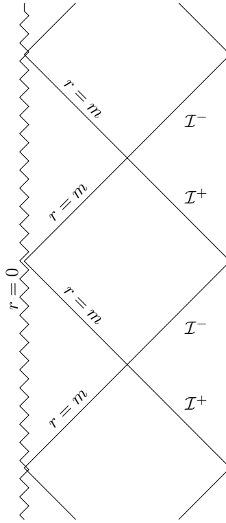
Figure 36: Penrose Diagram of the extremal Reissner-Nordström metric.
