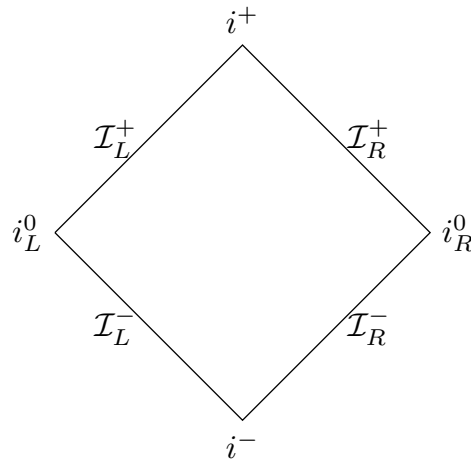
Figure 24: Penrose Diagram for (1+1)-dimensional Minkowski space
