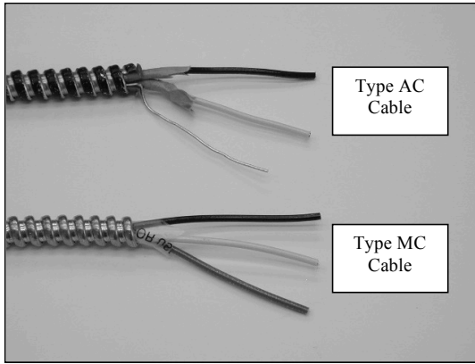
Photo No. 1. AC and MC cable
