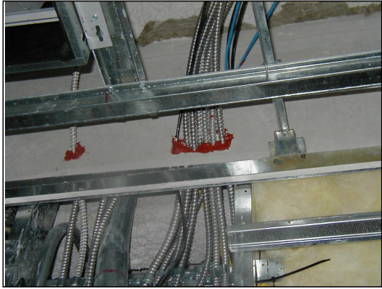
Photo No. 8. Firestopping through penetrations
