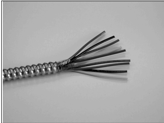
Photo No. 3. Multiple Neutral Conductors
