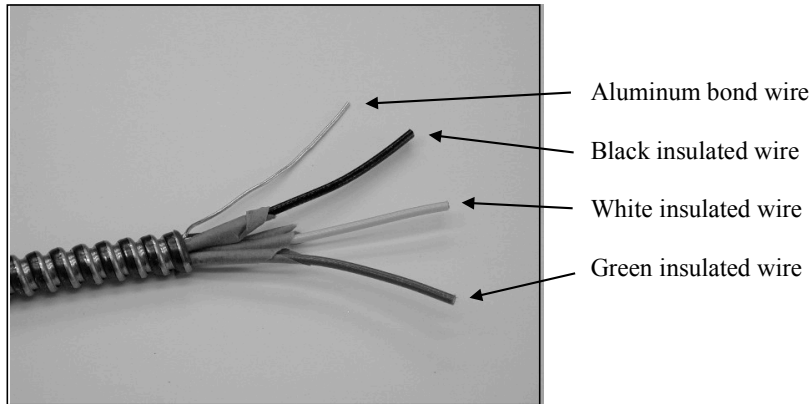
Photo No. 9. Type AC Health Care Cable
