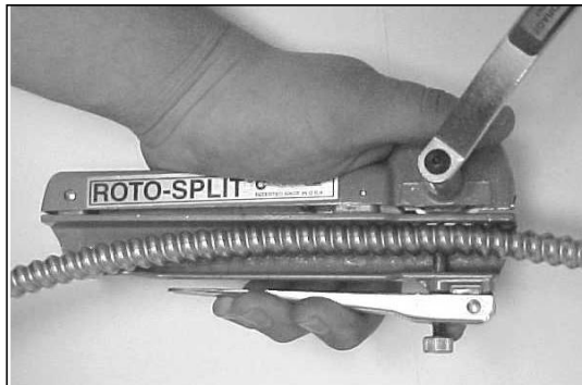
Photo No. 7. Roto Split
