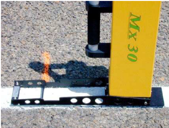
Figure 3-6. Handheld instrument prepared for retroreflectivity measurement.
