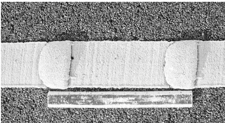
Figure 2-13. Typical raised-profile thermoplastic marking (overhead view).
