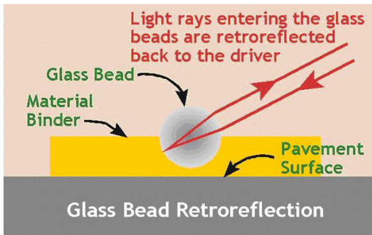
Figure 2-17. 2-17. Pavement-marking retroreflectivity using glass beads.
