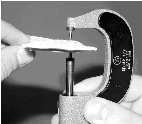
Figure 3-1. Needlepoint micrometer measuring thermoplastic sample.
