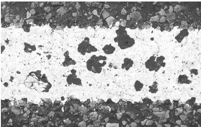
Figure 2-6. Asphalt boiling through hot thermoplastic.
