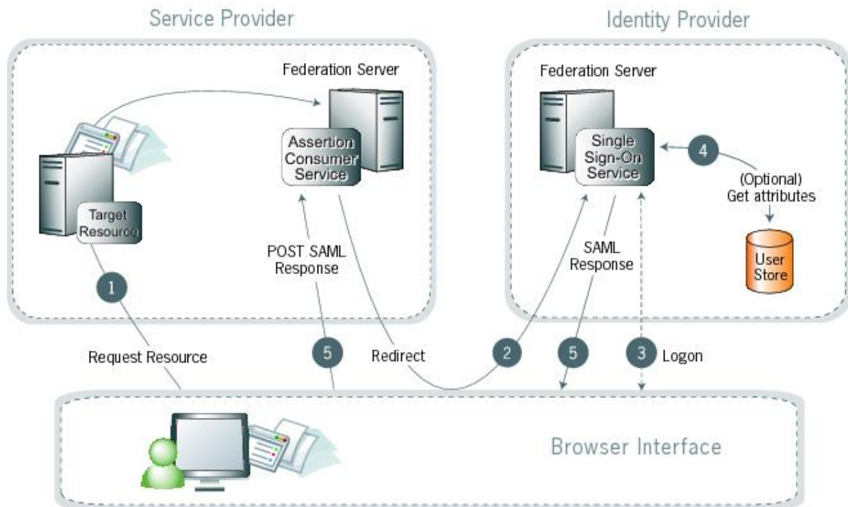
Figure 8: SP-initiated SSO: redirect/POST
