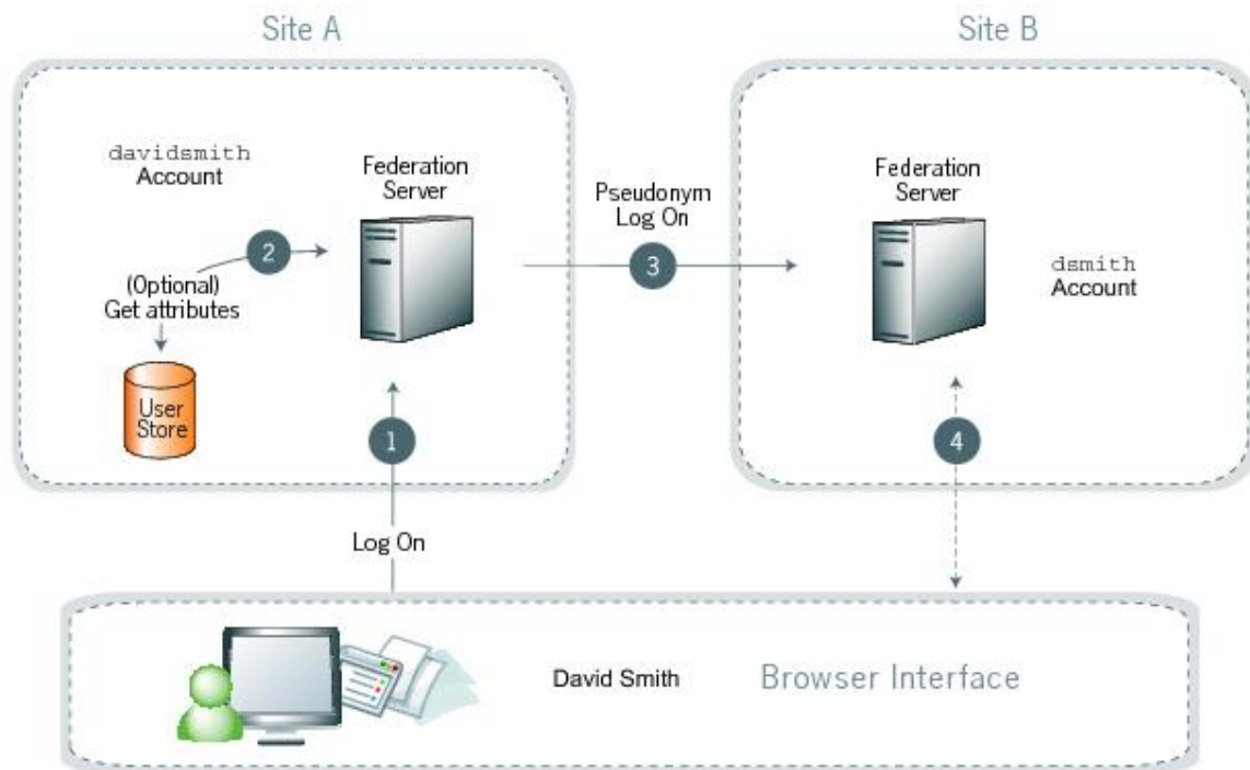
Figure 15: Account linking
