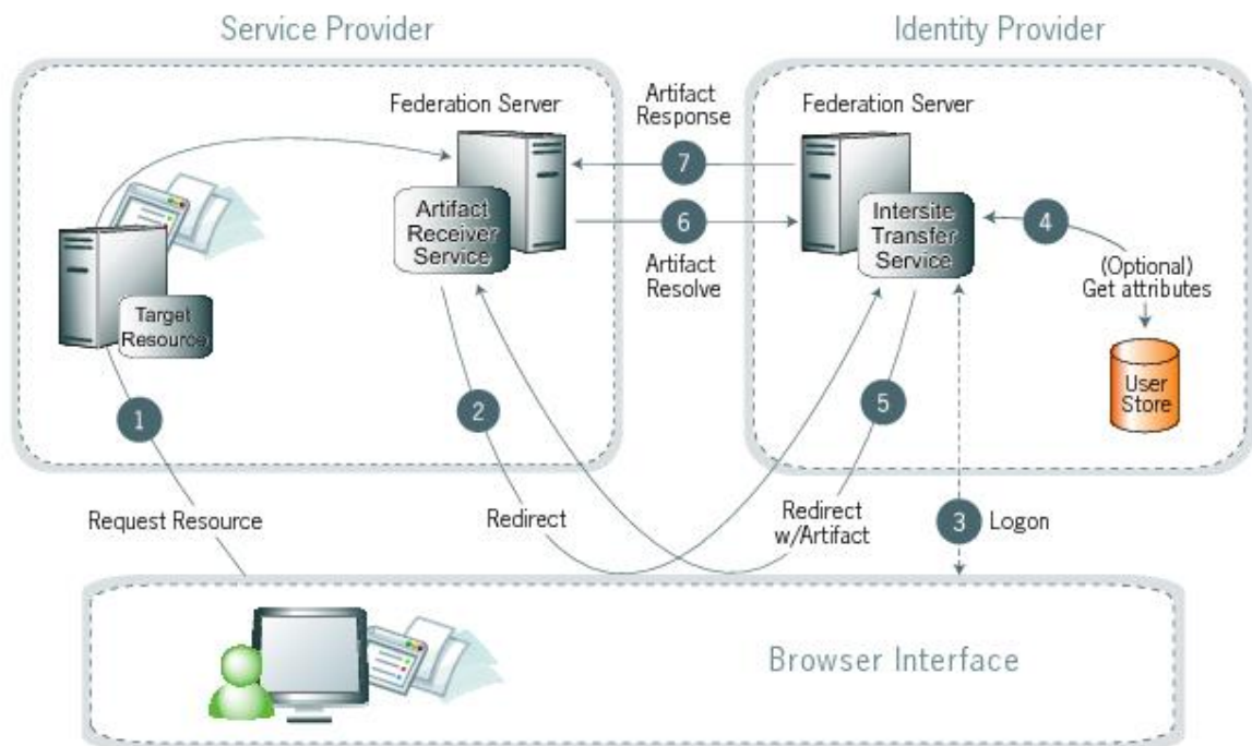
Figure 6: SP-initiated SSO
