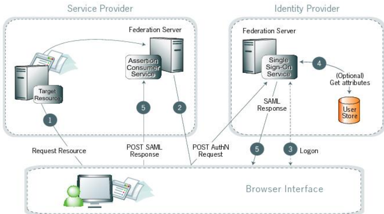
Figure 7: SP-initiated SSO: POST/POST
