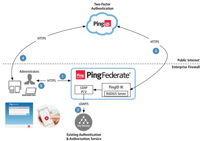
Figure 25: Multifactor Console Authentication using PingID
