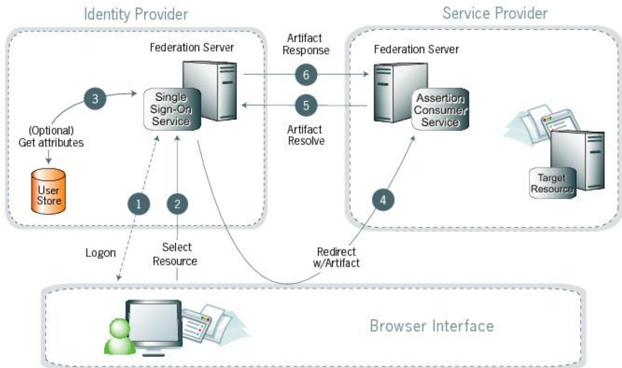
Figure 14: IdP-initiated SSO: artifact
