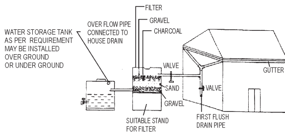
Fig. 2.1 Storing rain water for direct use method.
