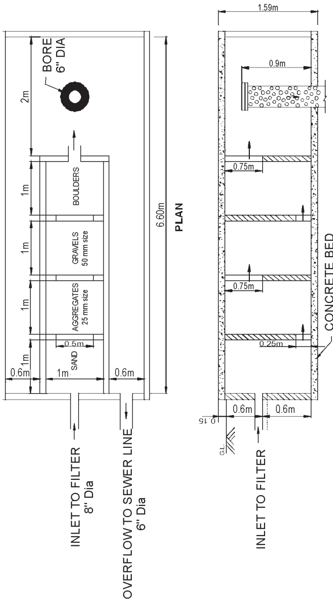
Fig. 4.3 Details of settlement tank / filter for Rain Water Harvesting
