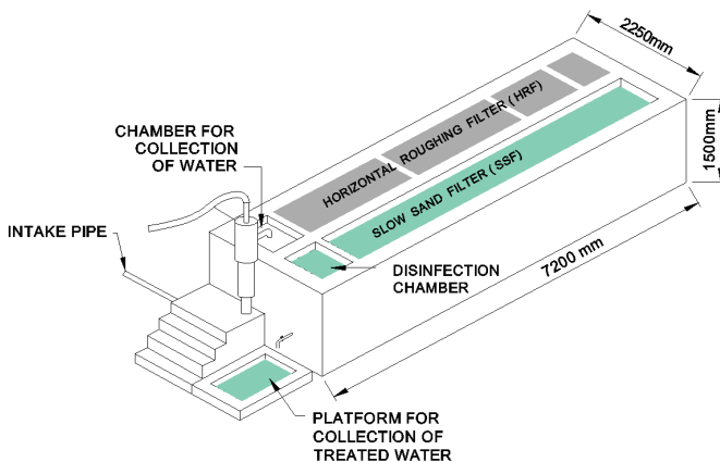
Fig. 2.12 Horizontal roughening filter and slow sand filter
