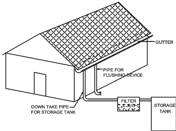
Fig. 2.6 First flushing device
