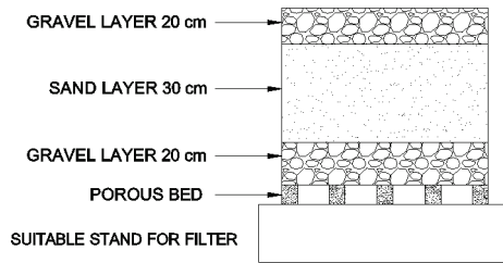
Fig. 2.8 Sand filter
