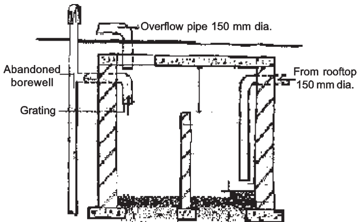
Fig. 2.15 Settlement tank
