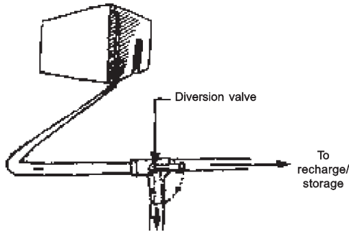
Fig. 2.7 First flushing device.
