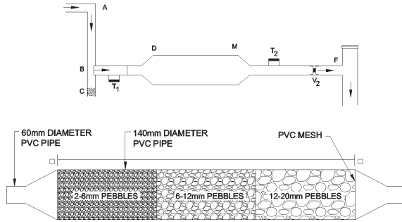
Fig. 2.10 Dewas filter
