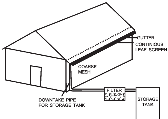
Fig. 2.5 Leaf screen
