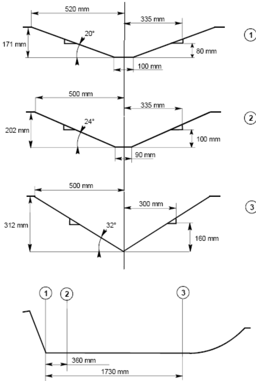
Hull profile
