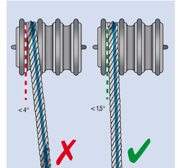
Fig. 37: Lateral deflection when running over a sheave
