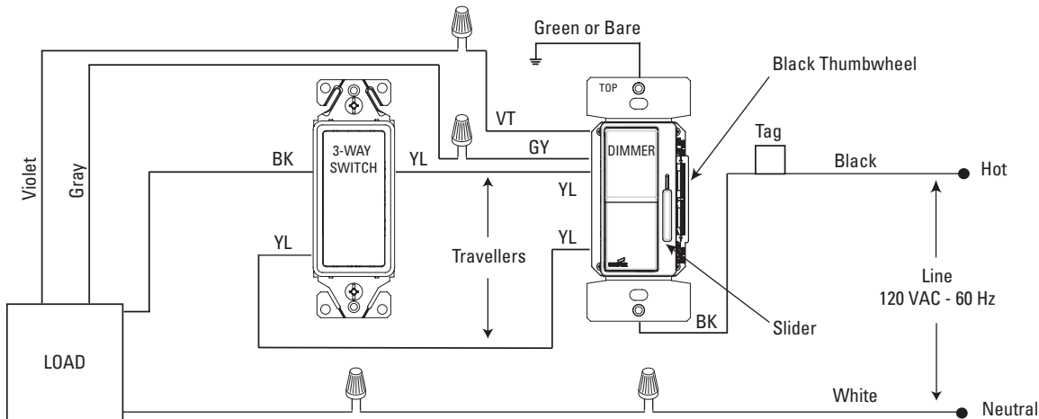
FIGURE 2: 3-WAY WIRING DIAGRAM
