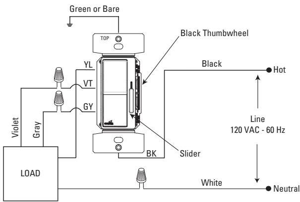
FIGURE 1: SINGLE-POLE WIRING DIAGRAM
