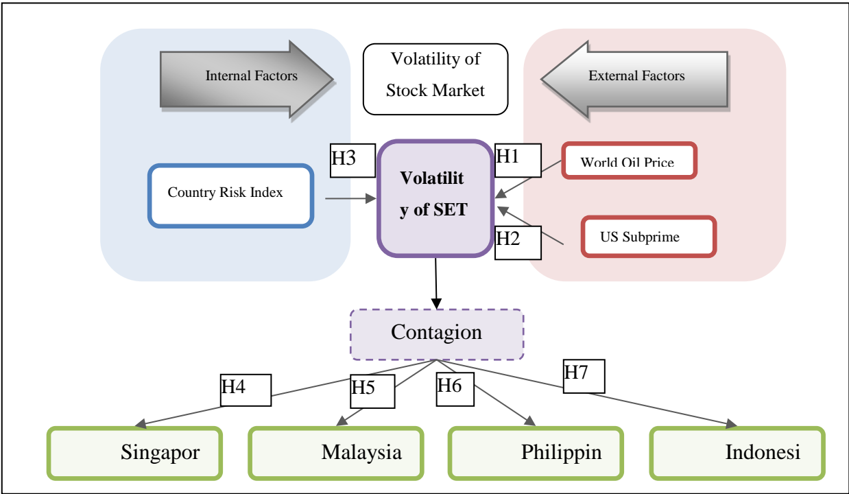
Figure 3.1: Conceptual framework.
