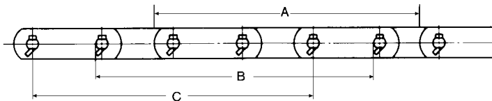
Fig. 15-5 Places to Measure Chain Elongation
