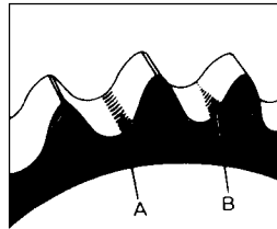
Fig. 9-4 Areas to Check for Sprocket Wear
