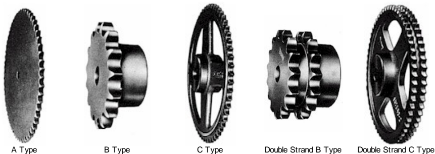
Fig. 5-1 Sprocket Types
