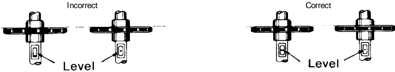
Fig. 6-1 Shaft Alignment
