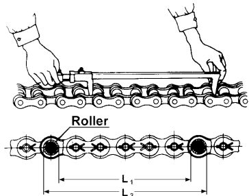
Fig. 9-5 Measuring Chain Elongation
