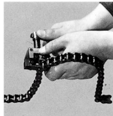
Fig. 4-5 Using the chain breaker
