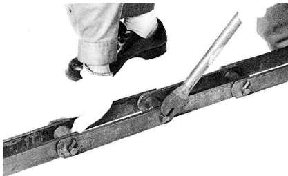
Fig. 11-3 Inserting New T-Pins or Cotter Pins
