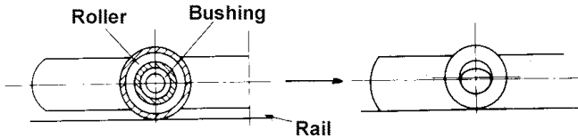
Fig. 15-1 Roller Wear
