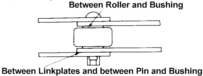
Fig. 13-1 Important Conveyor Chain Lubrication Points
