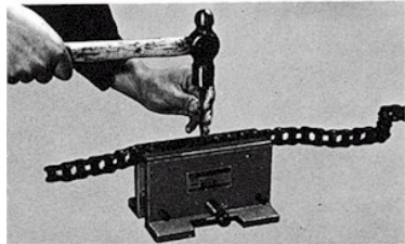
Fig. 4-1 Disconnecting RS Roller Chain
