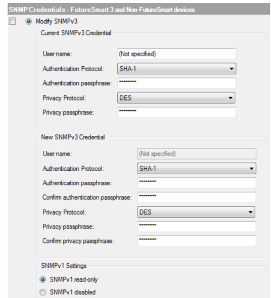
Figure 1—SNMP setup (single device)
