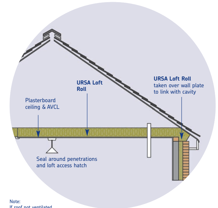
Figure 2 – LR Underlay
