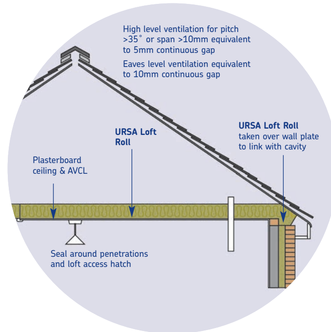
Figure 1 – HR Underlay
