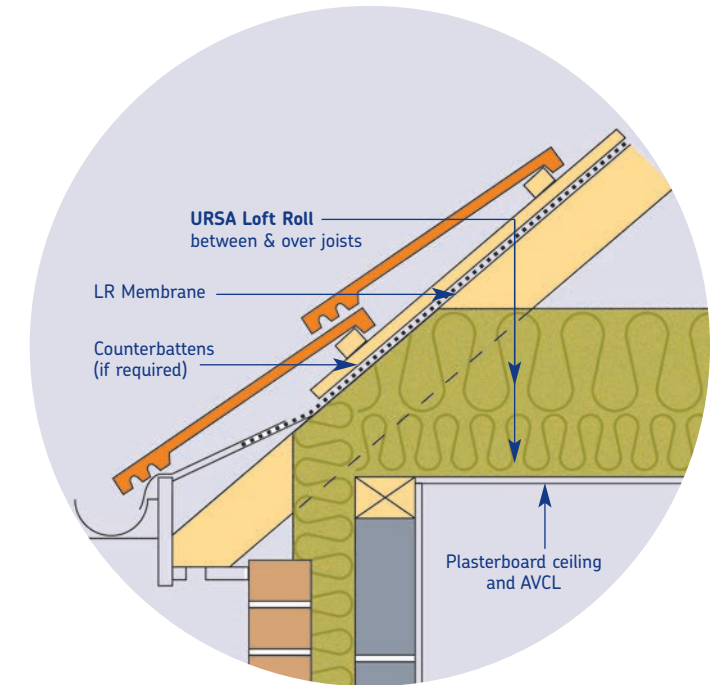
Figure 4 – Non-Ventilated Void
