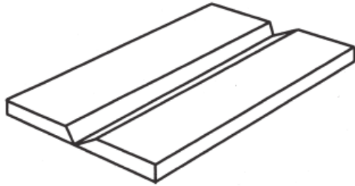
FLAT TEST POSITION 1G
