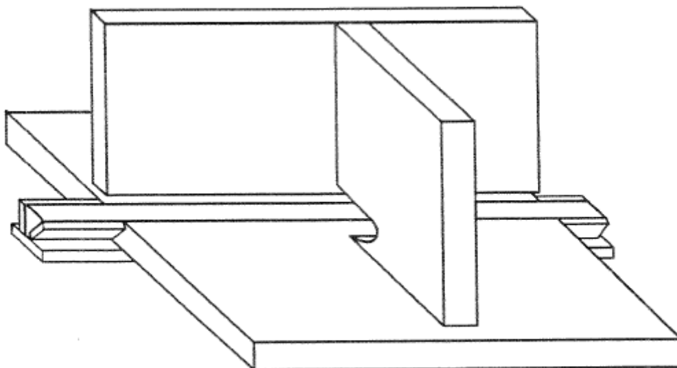
FIGURE 17-13.14.2 – TEST PLATE CONFIGURATION FOR OPTION B
