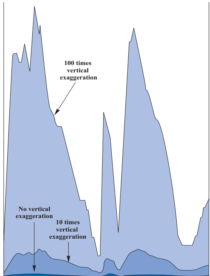
FIGURE 1-7 Most vertical profiles are vertically exaggerated. Topography appears progressively more distorted as the exaggeration increases. The relatively flat topography depicted in this figure looks like extremely rugged mountain chains with very steep slopes when it is plotted at a vertical exaggeration of 100 times. Most oceanographic profiles are plotted with vertical exaggerations greater than 100 times.
