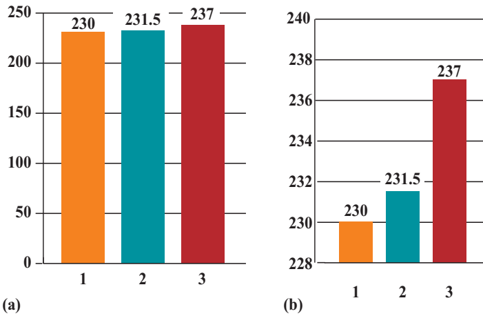
FIGURE 1-4 These two bar charts show the same data but use different y-axis ranges. Notice that they give very different impressions about the differences among the three values.
