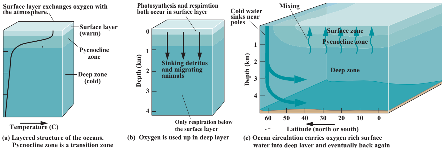
FIGURE 1-2 Oxygen concentration in ocean water is controlled by both physical and biological processes. (a) The oceans consist of two main layers, a warm surface layer, and a cold deep layer, with a transition zone called the pycnocline zone between them. (b) Surface layer water is well mixed and in contact with the atmosphere and its oxygen concentration is primarily controlled by gas exchange with the atmosphere. Photosynthesis by marine life in this layer converts carbon dioxide to organic matter and releases oxygen but this is offset by respiration that converts oxygen to carbon dioxide. Respiration also occurs in the deep layer, fueled by organic material (detritus) and animals that migrate vertically, but there is no photosynthesis and no contact with the atmosphere so respiration continuously consumes oxygen in this deep layer and the longer the water remains in the deep layers the less oxygen it contains (c) The deep layer water is continuously replenished by sinking of cold water in some near polar regions and then circulates through the oceans while being slowly mixed upward, eventually into the surface layer again. The pycnocline provides a barrier that inhibits mixing so the upwards mixing process is slow.
