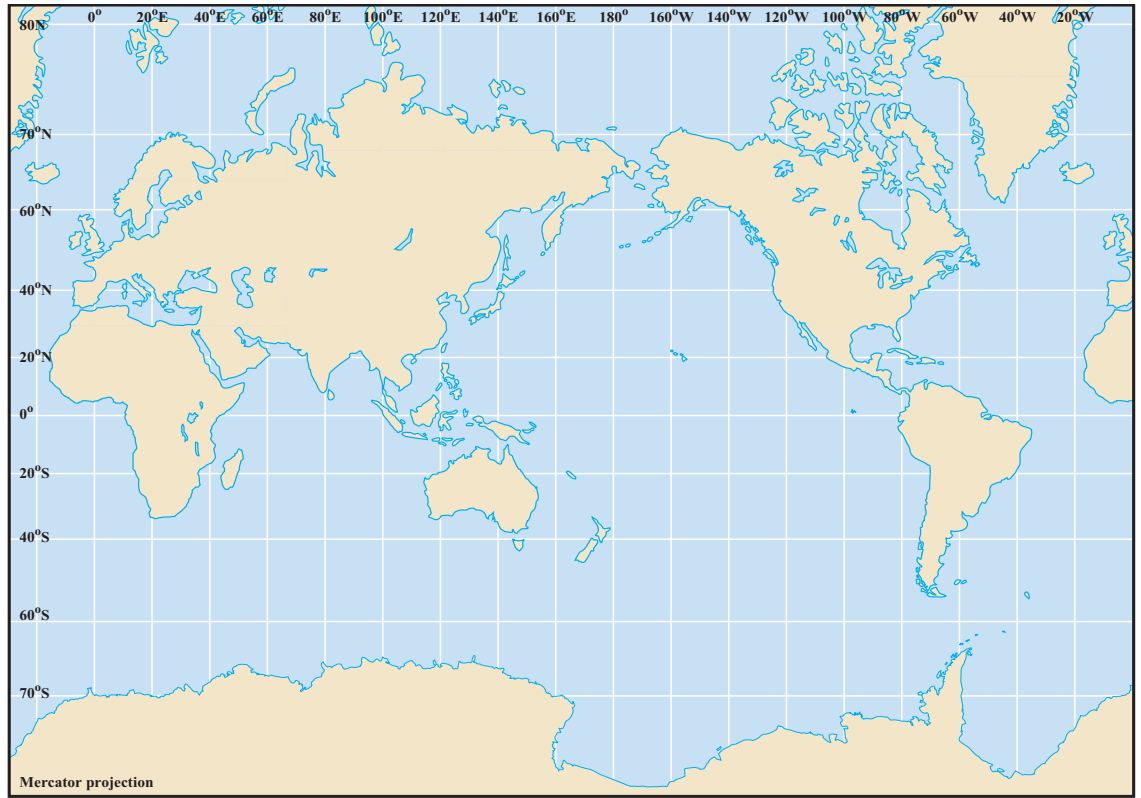
FIGURE 1-9 Typical map projections. (a) Mercator projection. Note that the map is cut off, so the higher latitudes near 90°N and 90°S are not shown. The reason is that the shape and area distortions introduced by this projection increase rapidly with latitude near the poles. (b) Goode’s interrupted projection. This projection preserves relative areas and shows each of the oceans without interruption. However, it distorts the shapes of the continents. (c) Robinson projection. This projection preserves none of the four desirable characteristics perfectly, but it is a good approximation for many purposes.
