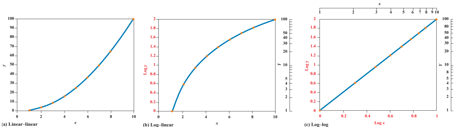
FIGURE 1-5 A simple nonlinear relationship is plotted in three different ways to show how logarithmic scales can change the apparent nature of the relationship between the two variables: (a) a linear-linear plot, (b) a log-linear plot, (c) a log-log plot.
